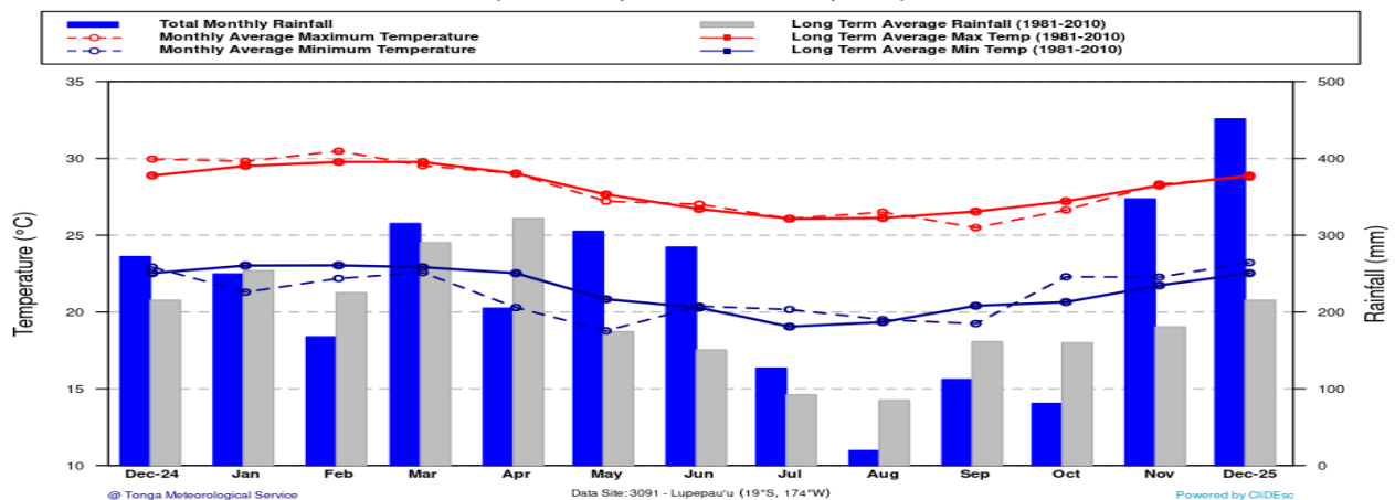
Lupepau'u (3091) - Temperature & Rainfall for the last 13 Months (December, 2024 - December, 2025)
