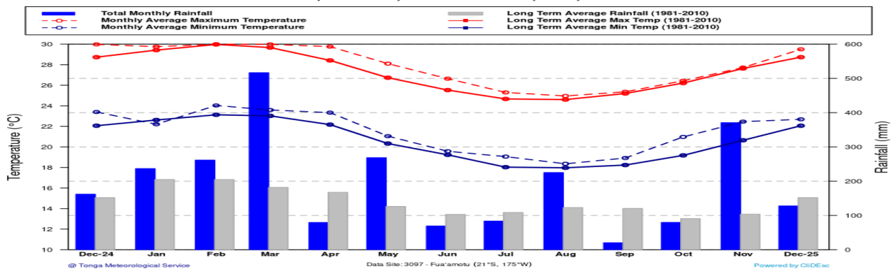
Fua'amotu (3097) - Temperature & Rainfall for the last 13 Months (December, 2024 - December, 2025)
